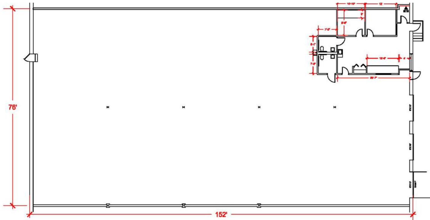
BUILDING KEY PLAN
